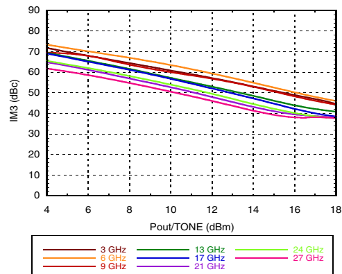
Output IM3 @ Vdd = 9V
