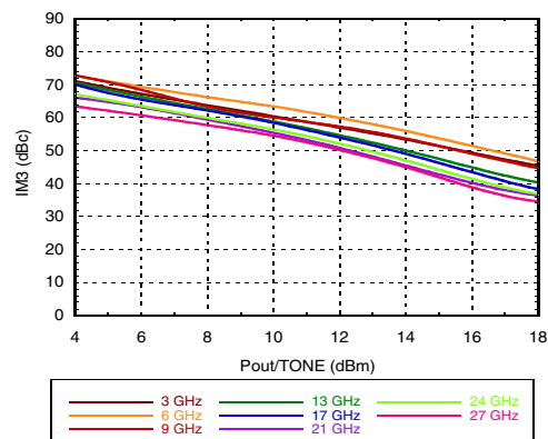
Output IM3 @ Vdd = 11V
